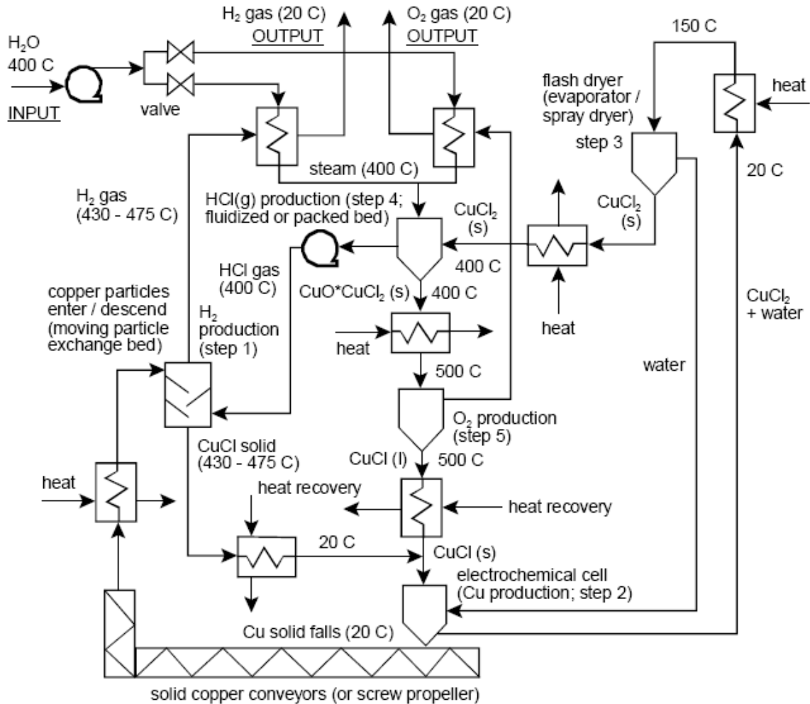
Fig. 1.1: Schematic of copper-chlorine cycle for hydrogen production, Ref. [3].
